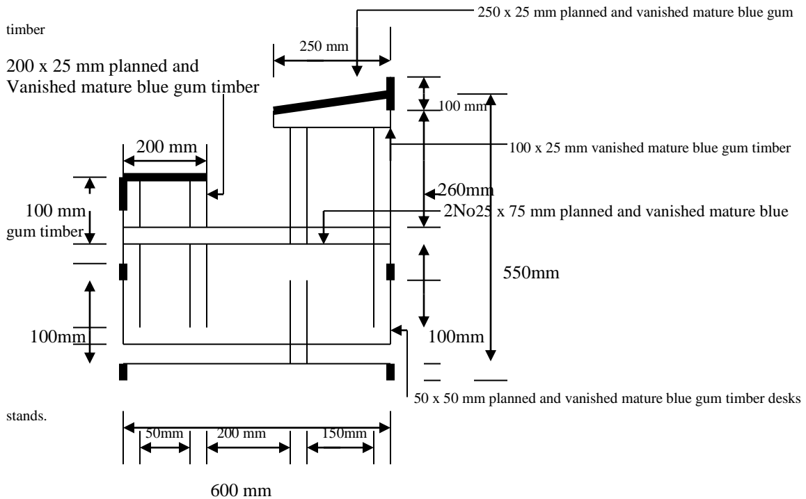
Side elevation 01
